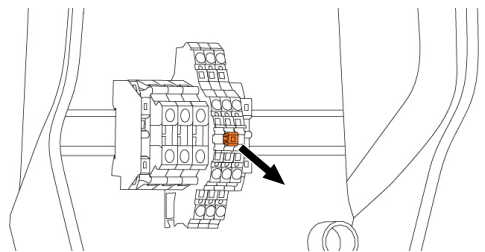
Fig. 10: Remove jumper
