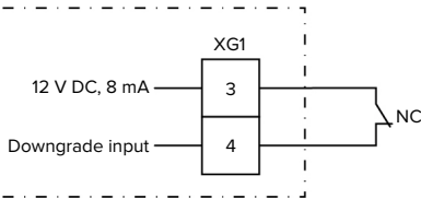
Fig. 11: Schematic circuit diagram: Connection of an external switching contact
