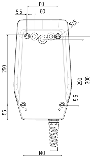
Afb. 6: Boormaten [mm]
